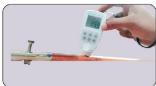
Coating Thickness Test Clause 9.6.1 (UL 467).
